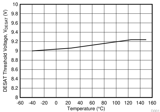
Figure 6-24. V_{DESAT} DESAT Threshold Voltage vs Temperature
