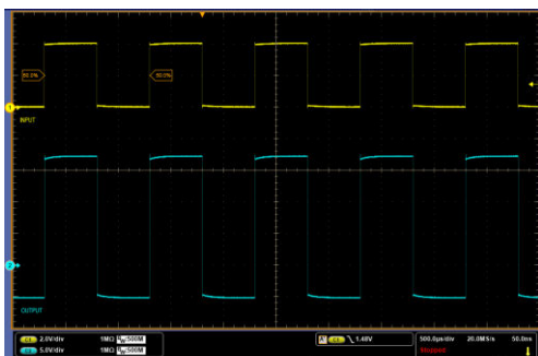
Figure 9-14. PWM Input (Yellow) and Driver Output (Blue)
