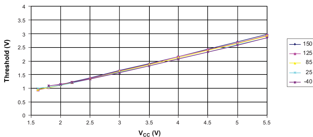
Figure 30-39. I/O Pin Input Threshold Voltage versus V_{CC} ( V_{IH} , I/O Pin read as '1')
