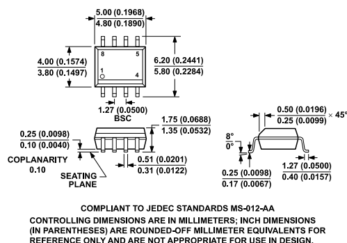
Figure 12. 8-Lead Standard Small Outline Package [SOIC_N] Narrow Body (R-8) Dimensions shown in millimeters and (inches)
