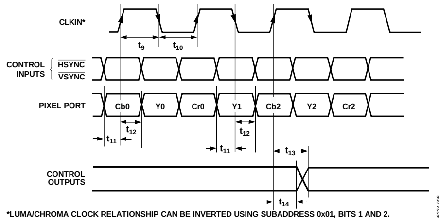
Figure 8. ED/HD-DDR Input, 8-/10-Bit 4:2:2 YCrCb ( \overline{\text{HSYNC}} / \overline{\text{VSYNC}} ), Input Mode 010
