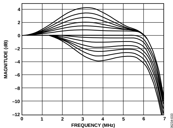
Figure 35. SD Luma SSAF Filter, Programmable Responses
