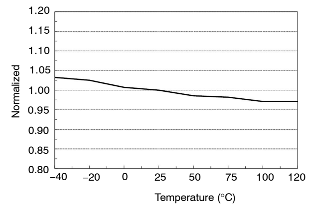
Figure 21. V_{OCP} vs. Temperature
