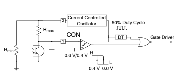
Figure 42. Pulse-Skipping Circuit
