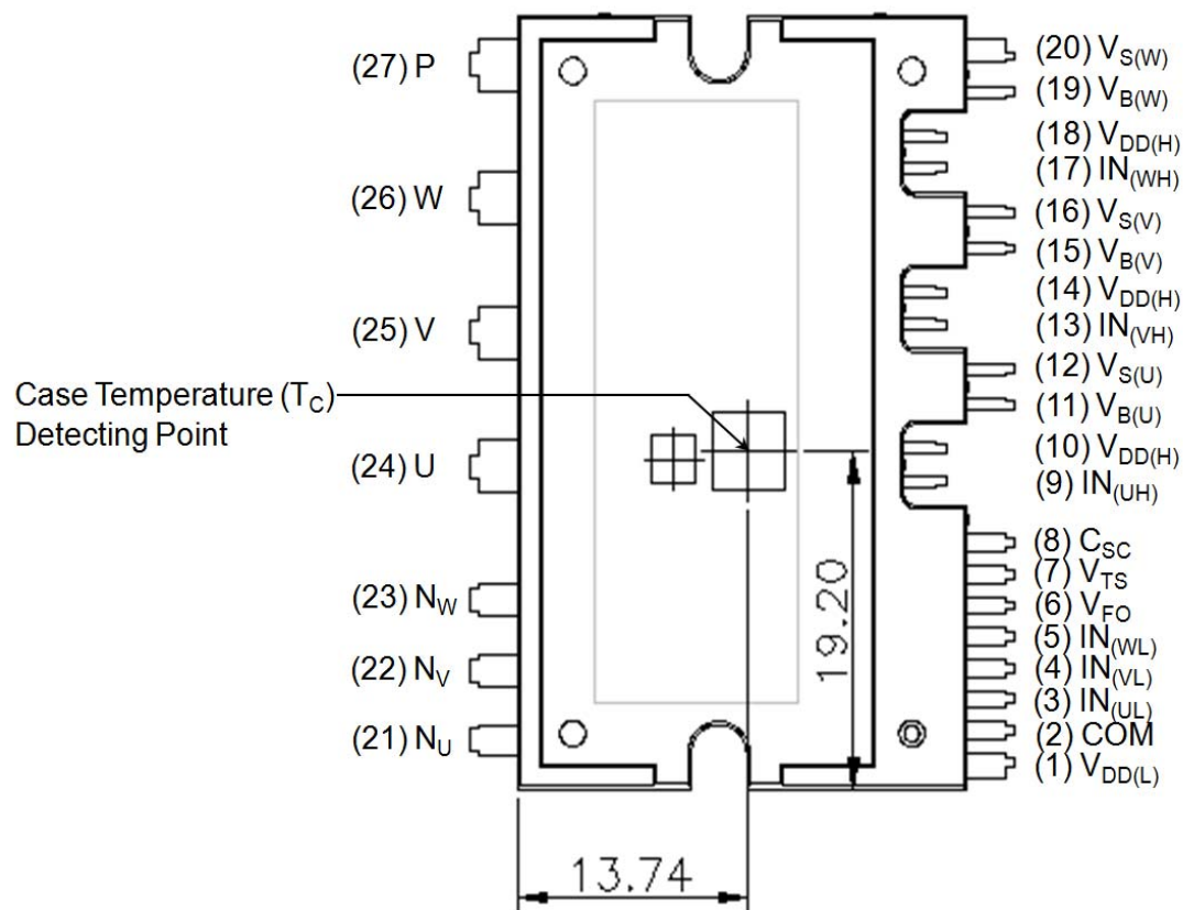
Figure 2. Top View
