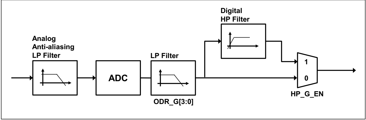
Figure 8. Gyroscope chain
