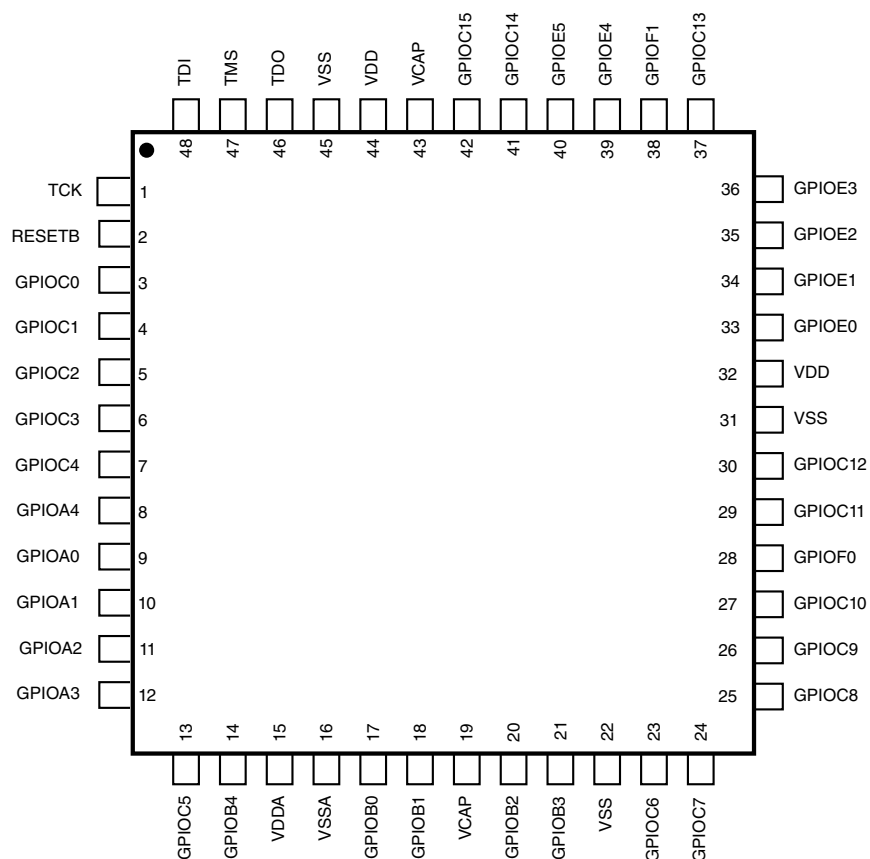
Figure 23. 48-pin LQFP
