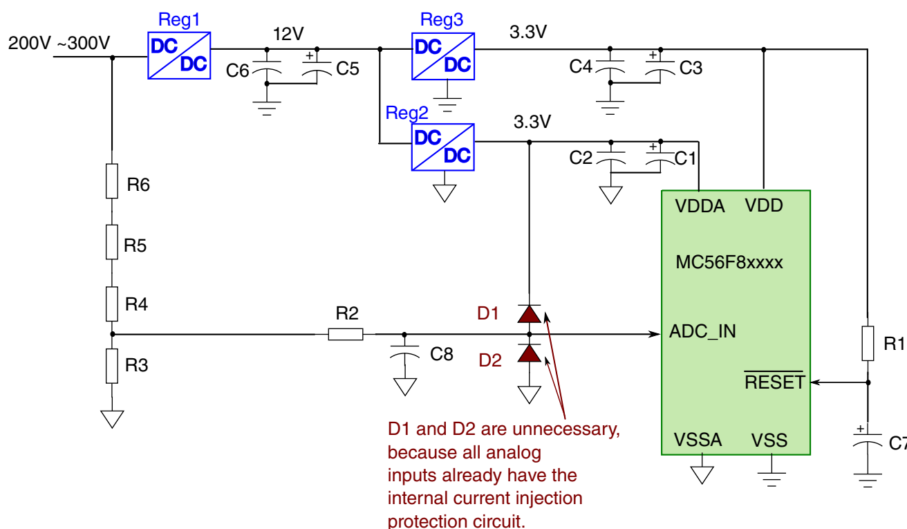
Figure 21. Protection Circuit Example
