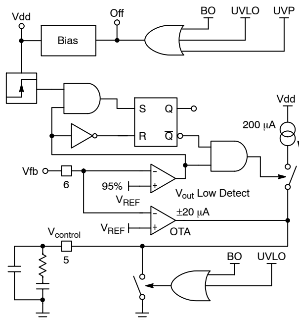
Figure 42. Soft Start Block Diagram
