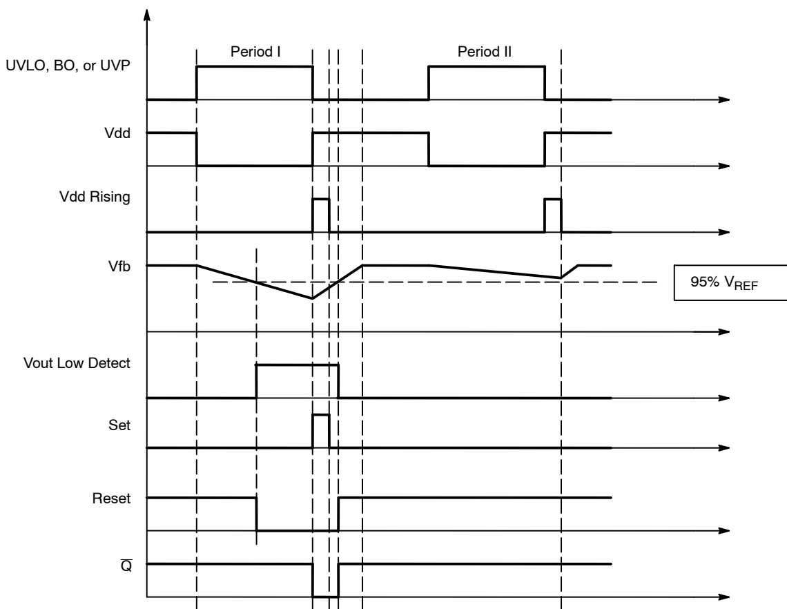
Figure 43. Soft Start Timing Diagram
