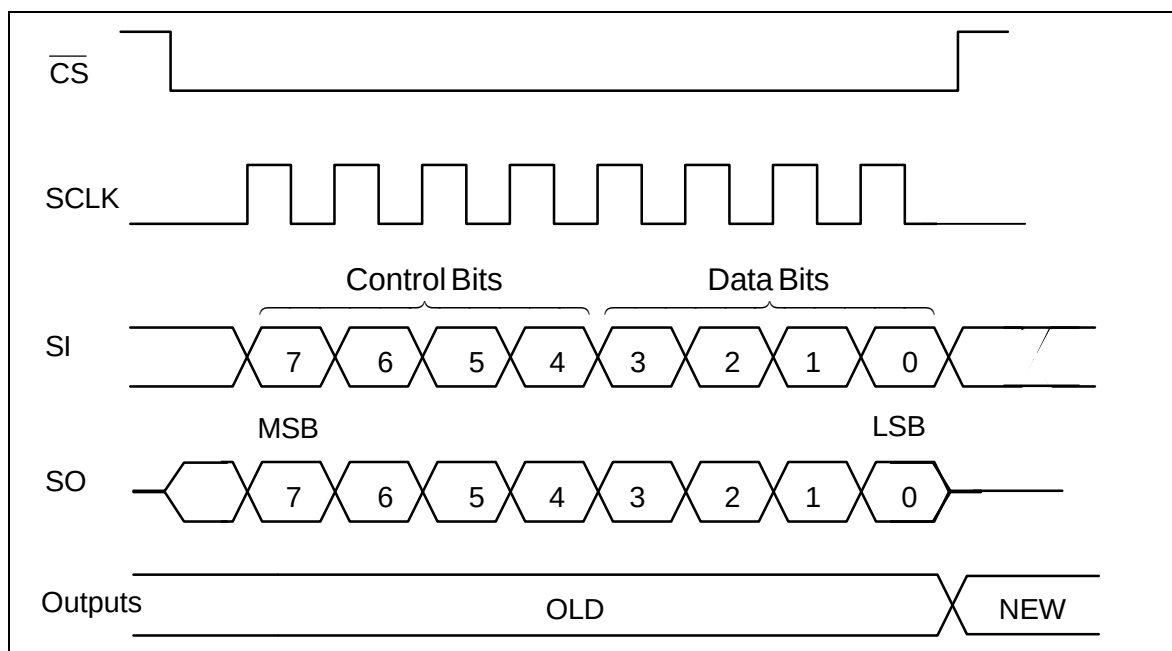
Figure 2: Serial Interface
