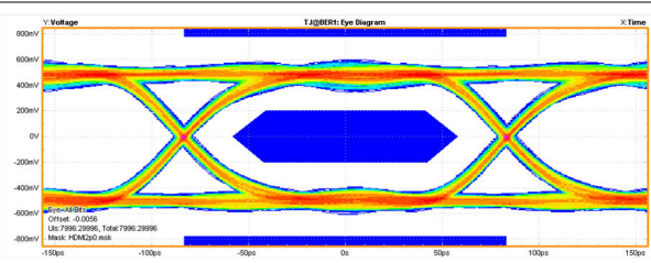
Figure 7-9. 6-Gbps HDMI 2.0 (TP1) Eye Diagram TPD6E05U06
