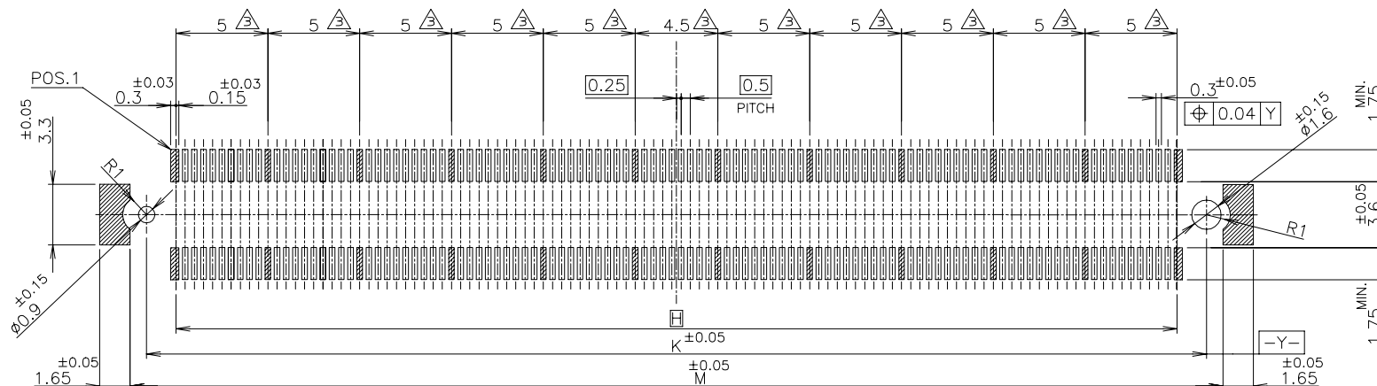
REFERENCE P.C.BOARD LAYOUT
