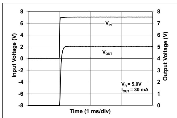
FIGURE 2-37: Start-up Response.
