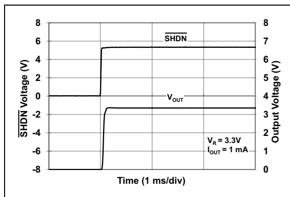
FIGURE 2-40: SHDN Response.
