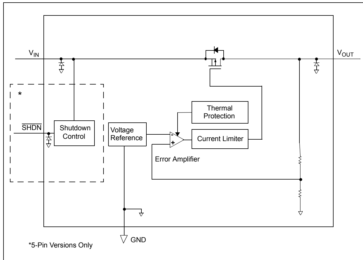
FIGURE 4-1: Block Diagram.
