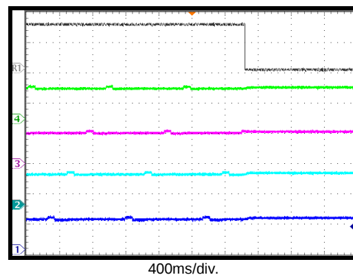
Shutdown through EN No PD connection
