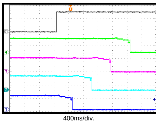
Start-Up through EN Class 4 PD connection
