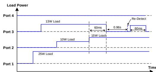
Figure 12: PMAX Power Management at 50W
