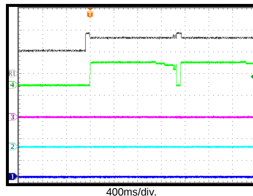
PMAX Limit Triggered (10)
