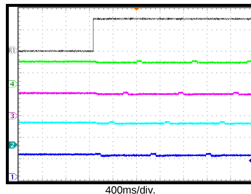
Start-Up through EN No PD connection
