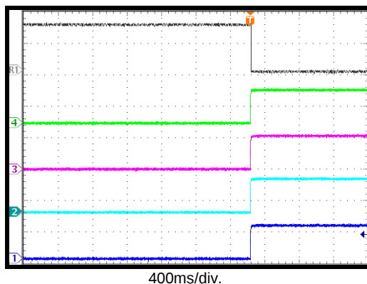
Shutdown through EN Class 4 PD connection
