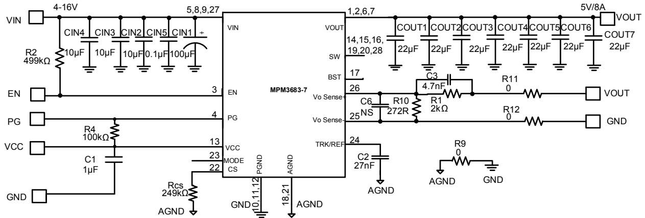
Figure 8: 12V IN 5V/8A Output, CCM1000KHz
