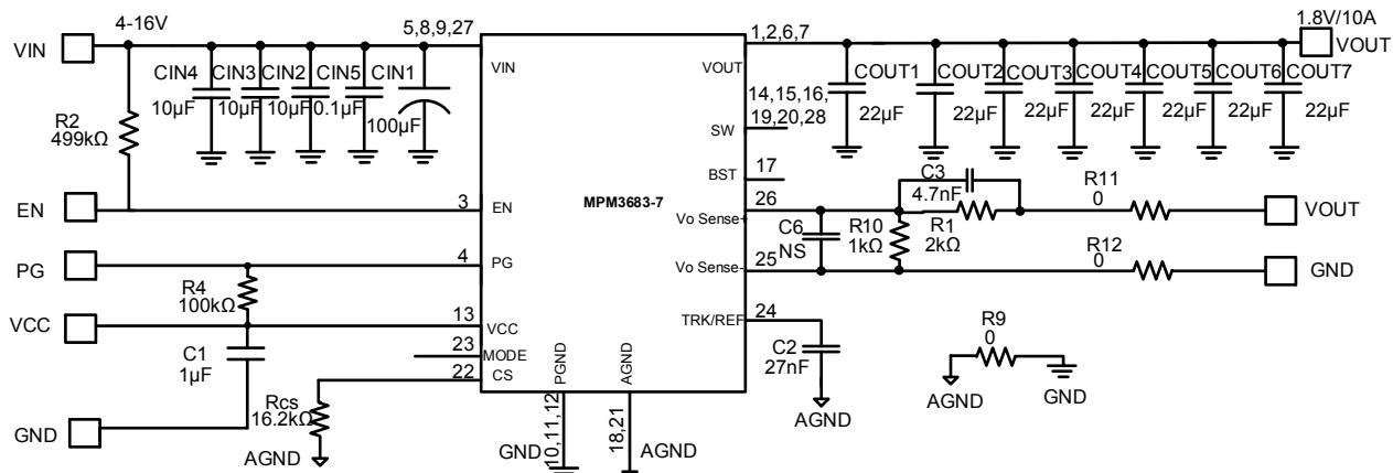
Figure 10: 12V IN 1.8V/10A Output, CCM1000KHz
