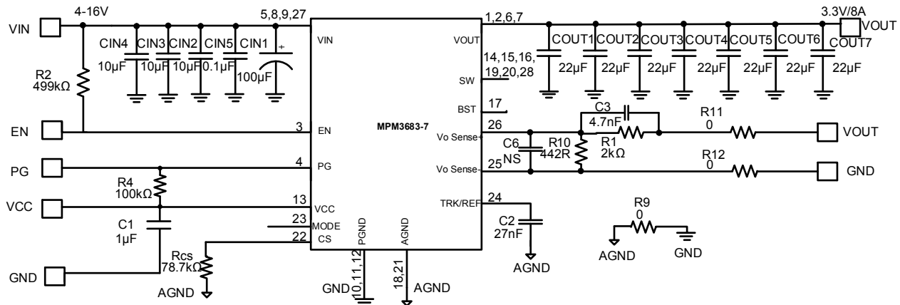
Figure 9: 12V IN 3.3V/8A Output, CCM1000KHz
