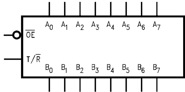
Figure 1. Logic Symbol
