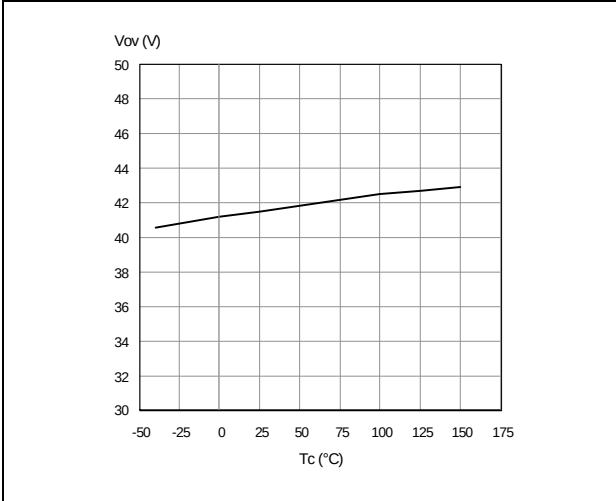
Figure 17. Overvoltage shutdown
