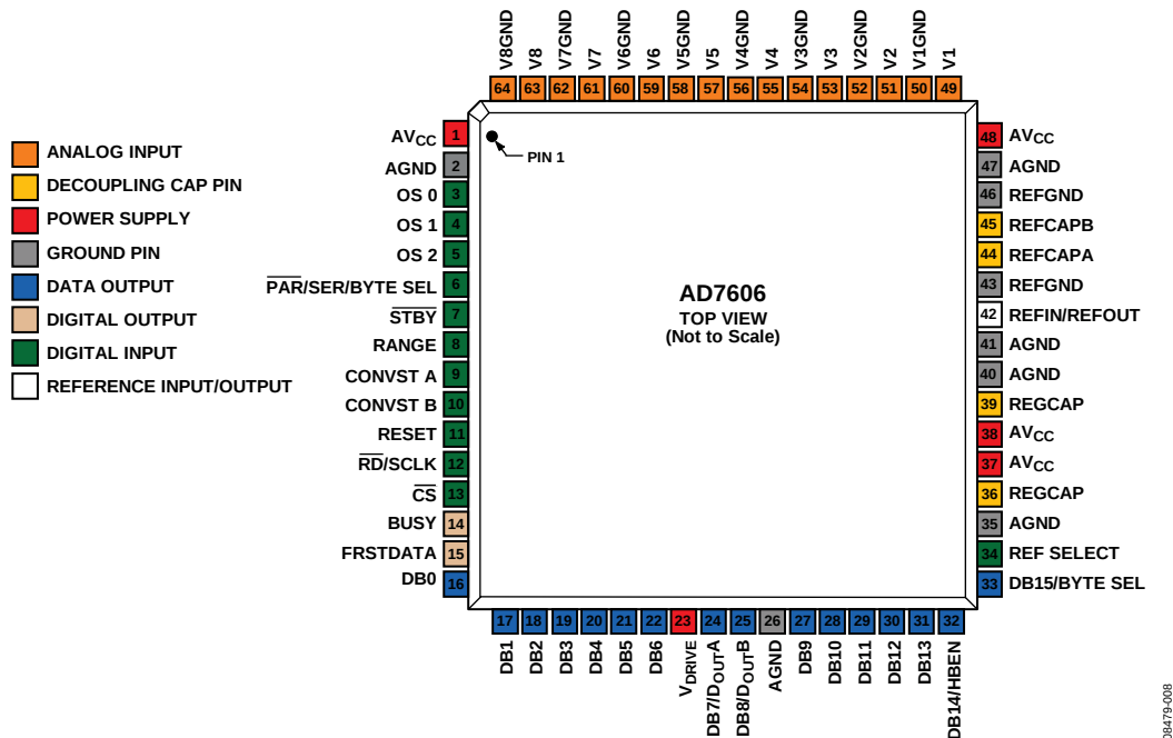
Figure 8. AD7606 Pin Configuration
