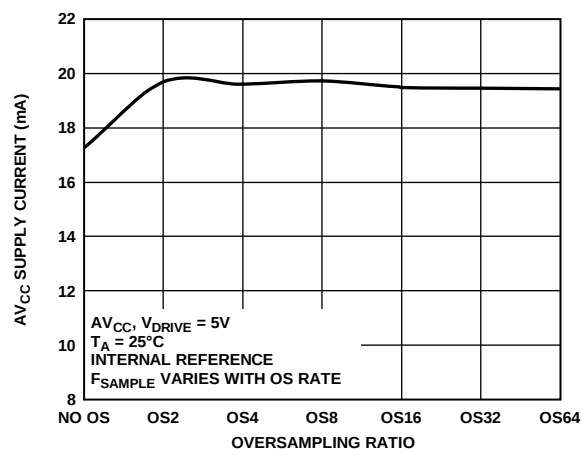
Figure 32. Supply Current vs. Oversampling Rate
