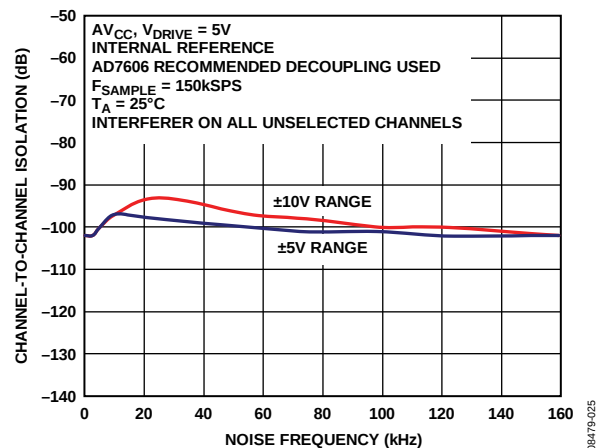
Figure 28. Channel-to-Channel Isolation
