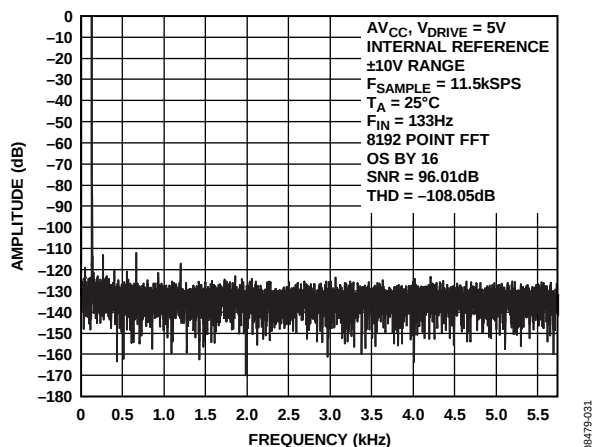
Figure 13. FFT Plot Oversampling By 16, \pm 10 V Range
