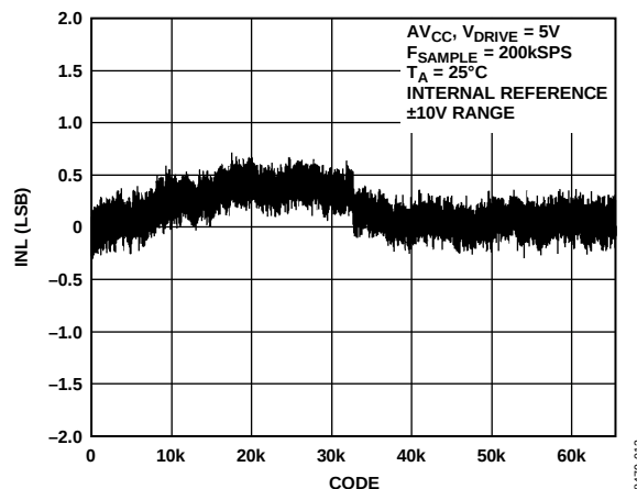
Figure 14. AD7606 Typical INL, \pm 10 V Range
