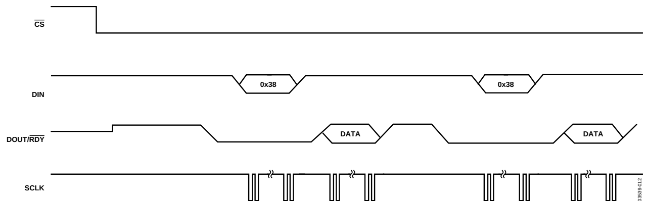
Figure 12. Continuous-Conversion Mode
