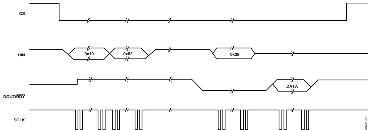
Figure 11. Single Conversion
