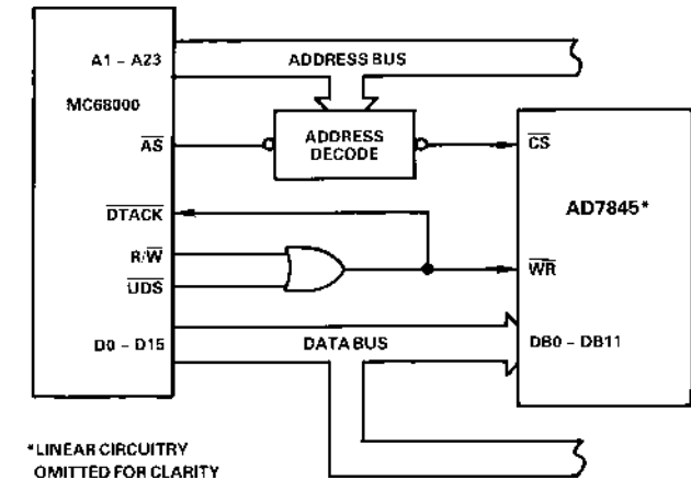
Figure 19. AD7845 to MC68000 Interface
