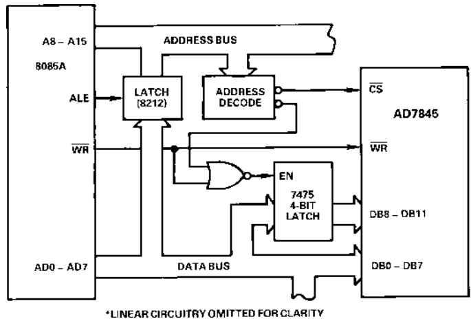
Figure 22. 8085A Interface
