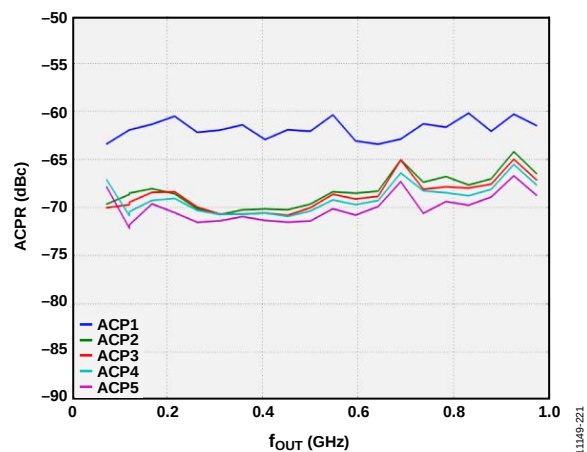
Figure 116. Eight-Carrier ACPR vs. f_{OUT}
