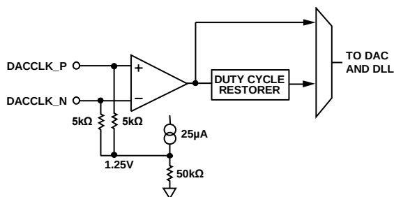
Figure 147. Clock Input
