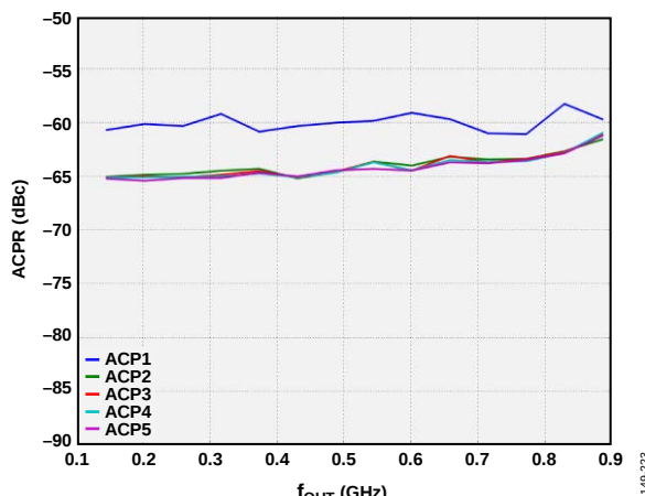
Figure 118. 32-Carrier ACPR vs. f_{OUT}
