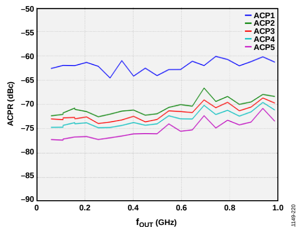
Figure 115. Four-Carrier ACPR vs. f_{OUT}
