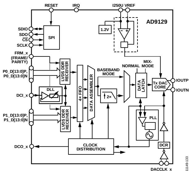
Figure 128. Functional Block Diagram of the AD9119/AD9129
