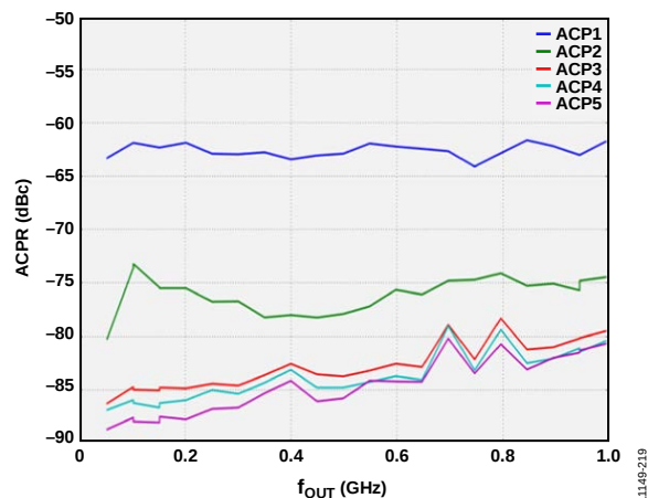
Figure 114. Single-Carrier ACPR vs. f_{OUT}
