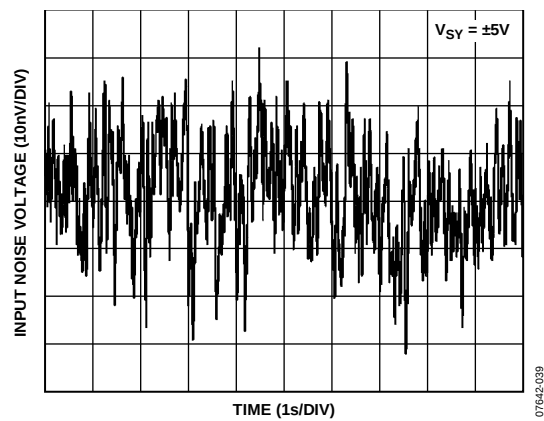
Figure 50. 0.1 Hz to 10 Hz Noise
