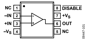
Figure 1. 8-Lead SOIC (ADA4897-1)
