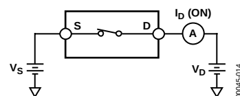
Figure 14. On Leakage
