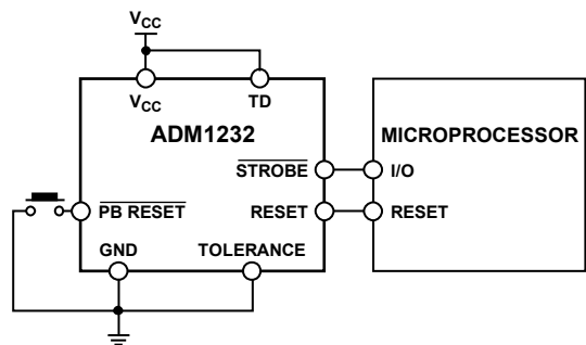
Figure 6. Typical Push-Button Reset Application
