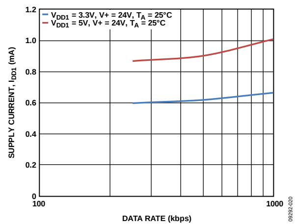
Figure 14. Supply Current ( I_{DD1} ) vs. Data Rate ( V_{DD1} = 3.3V, 5V ; V_+ = 24V )
