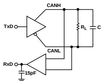
Figure 25. Switching Characteristics Measurements
