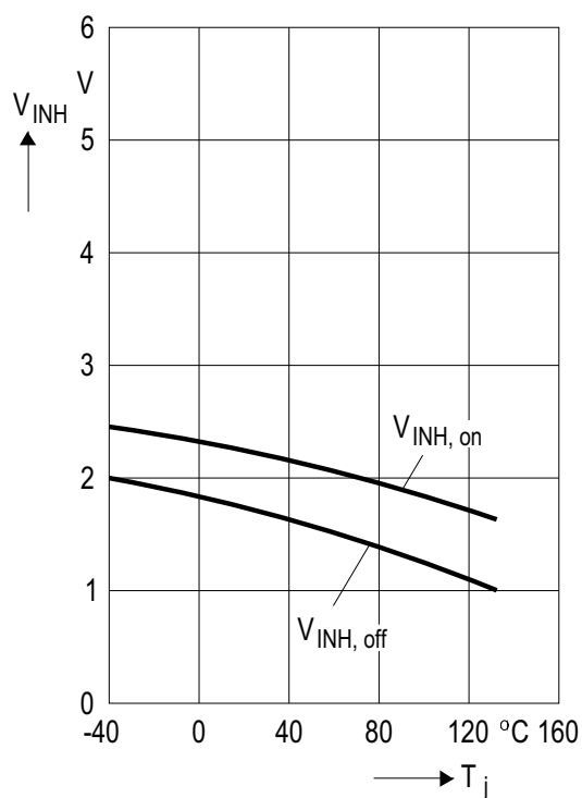
Inhibit voltages V_{INH} versus junction temperature T_j
