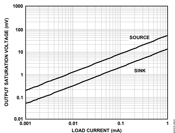
Figure 31. Output Saturation Voltage vs. Load Current V_S = 1.8\text{ V}
