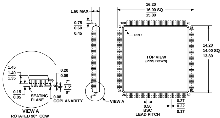
Figure 10. 100-Lead Low Profile Quad Flat Package [LQFP] (ST-100-1)
