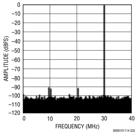
LTM9009-14: 8k Point FFT, f_{IN} = 30\text{MHz} , -1\text{dBFS} , 80Msps
