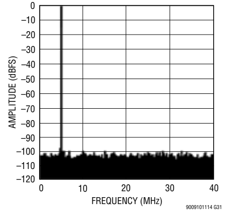
LTM9009-14: 8k Point FFT, f_{IN} = 5\text{MHz} , -1\text{dBFS} , 80Msps
