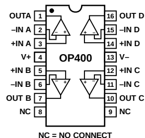
Figure 2. 16-Lead Standard Small Outline Package [SOIC_W]
