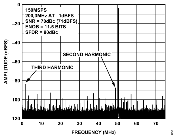
Figure 20. AD9640-150 Single-Tone FFT with f_{IN} = 200.3\text{ MHz}
