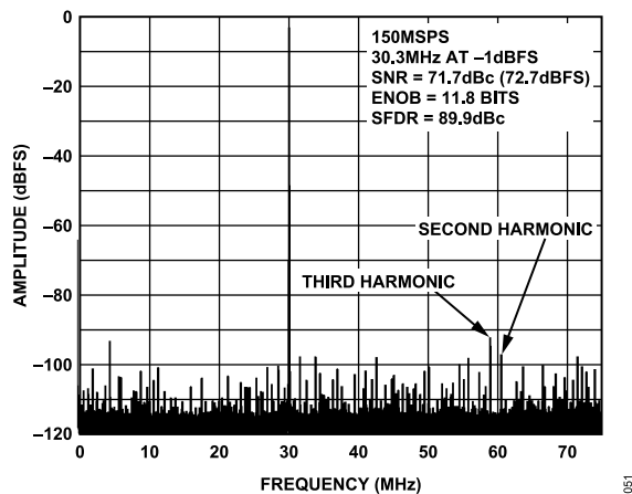
Figure 17. AD9640-150 Single-Tone FFT with f_{IN} = 30.3\text{ MHz}
