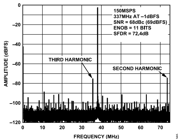
Figure 21. AD9640-150 Single-Tone FFT with f_{IN} = 337\text{ MHz}
