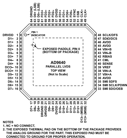
Figure 7. Pin Configuration, LFCSP LVDS (Top View)
