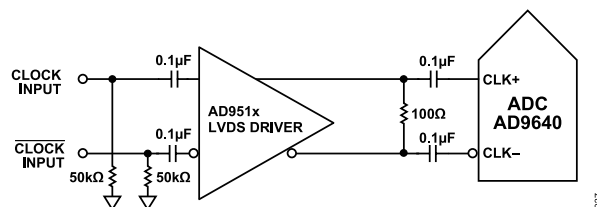
Figure 59. Differential LVDS Sample Clock (Up to 625 MHz)
