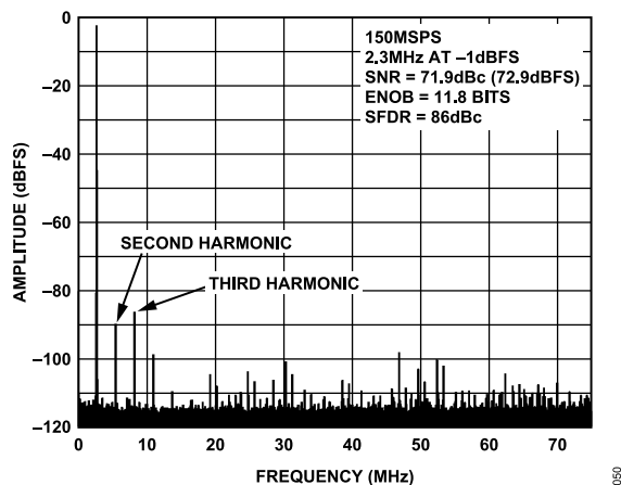
Figure 16. AD9640-150 Single-Tone FFT with f_{IN} = 2.3\text{ MHz}
