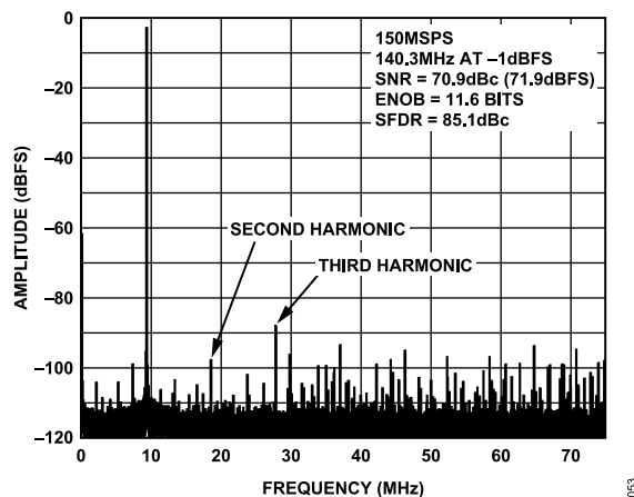
Figure 19. AD9640-150 Single-Tone FFT with f_{IN} = 140.3\text{ MHz}
