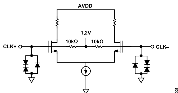
Figure 9. Equivalent Clock Input Circuit
