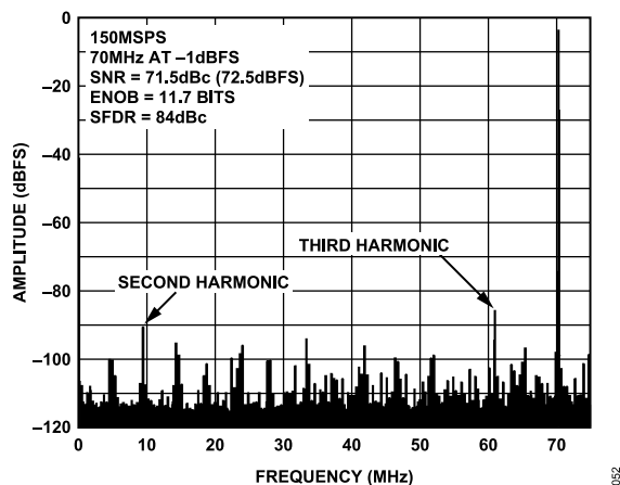
Figure 18. AD9640-150 Single-Tone FFT with f_{IN} = 70\text{ MHz}
