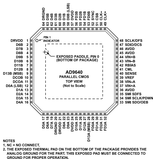
Figure 6. Pin Configuration, LFCSP Parallel CMOS (Top View)
