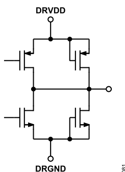
Figure 10. Digital Output
