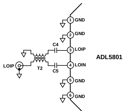
Figure 98. LO Interface
