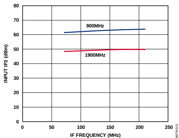
Figure 13. Input IP2 vs. IF Frequency
