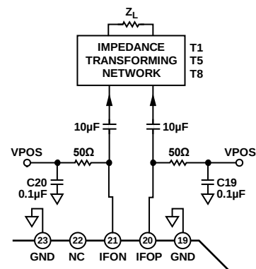
Figure 101. Resistive Bias Network to Downconvert Signals to Low Frequencies
