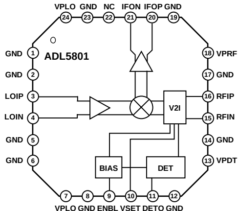
Figure 87. Block Diagram
