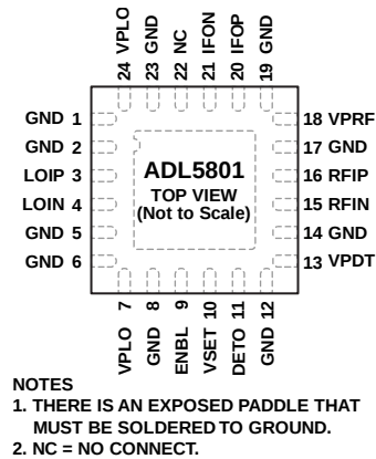
Figure 2. Pin Configuration
